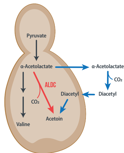
Figure 3: The addition of \alpha -acetolactate decarboxylase (ALDC) enzyme allows the direct breakdown of \alpha -acetolactate into flavorless acetoin (red lines) and prevents the formation and normal metabolism of diacetyl by the yeast cell (blue line).
